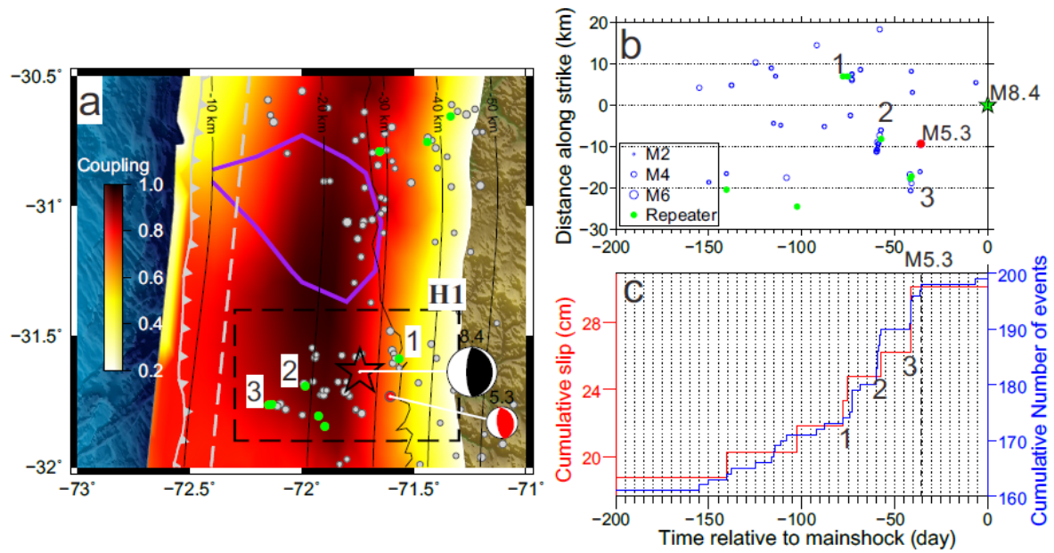
Figure 3. (a) A zoom-in map of region H1 (dashed rectangle, Figure 1b) with M \geq 3.0 seismicity (gray dots) and repeaters (green dots) within the last 200 days before the mainshock. The focal mechanisms of the M 5.3 event and the mainshock are from USGS NEIC. (b) shows the along-strike distance of seismicity within region H1 projected onto the gray dashed line in (a). (c) shows the cumulative number of events (blue) and aseismic slip (red). Note the quiescence of seismicity and repeaters after the M 5.3 event, lasting for \sim 36 days until the mainshock.
