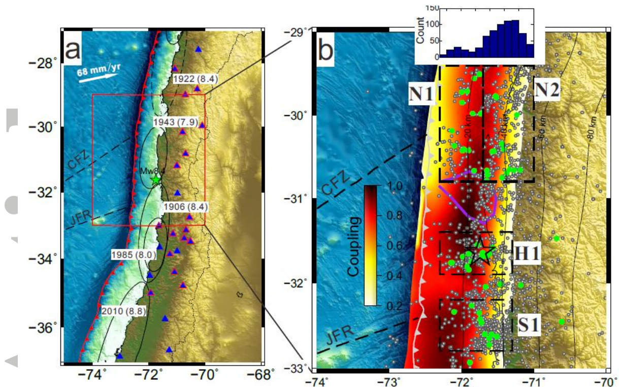
Figure 1. (a) Map showing the 27 stations used in the repeating earthquake analysis (blue triangles) and the subset of 17 stations used for matched-filter detection (blue triangles with red boundaries). The black and dashed ellipses denote maximal rupture zones of instrumental and historical megathrust earthquakes (Métóis et al., 2012). The green star denotes the epicenter of the 2015 M 8.4 Illapel mainshock. The plate convergence rate (68 mm/yr) is from Métóis et al. (2012). The two dashed lines indicate the Challenger fracture zone (CFZ) and Juan-Fernandez Ridge (JFR). (b). The gray dots show the locations of pre-mainshock events from the Centro Sismológico Nacional, Universidad de Chile (CSN). The green dots denote repeating earthquakes. N1, N2, H1 and S1 are four sub-regions for investigating the seismicity and aseismic-slip rates. The color scale denotes the model from Tilmann et al. (2016) which reflects plate coupling before the 2010 M 8.8 Maule earthquake. The purple curve denotes 5 m principal coseismic-slip contour of the 2015 M 8.4 Illapel earthquake from An and Meng (2016). The inset figure shows the histogram of the longitude of events within N1 and N2, which shows a bimodal distribution. The thin black contours show the Slab 1.0 geometry (Hayes et al., 2012).
