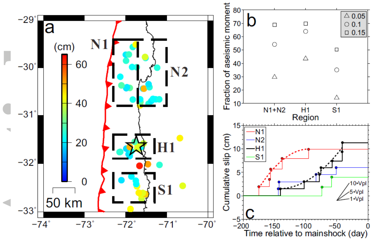
Figure 4. (a) The dots show the locations of repeating earthquake sequences before the 2015 Mw 8.4 Illapel event (black star), colored by the cumulative aseismic slip during the ~4-year period before the mainshock. (b) shows the proportion of aseismic moment among the total moment (seismic + aseismic) under the assumption of different sizes of grids around repeaters (0.05°, 0.1° and 0.15°, Figure S14). (c) shows the comparison of aseismic-slip series within the last 200 days. The dashed lines are the quadratic fits of the cumulative aseismic slip for region N1 and H1. The plate convergence rate ( V_{pl} ) is 68 mm/yr (Métois et al., 2012).
