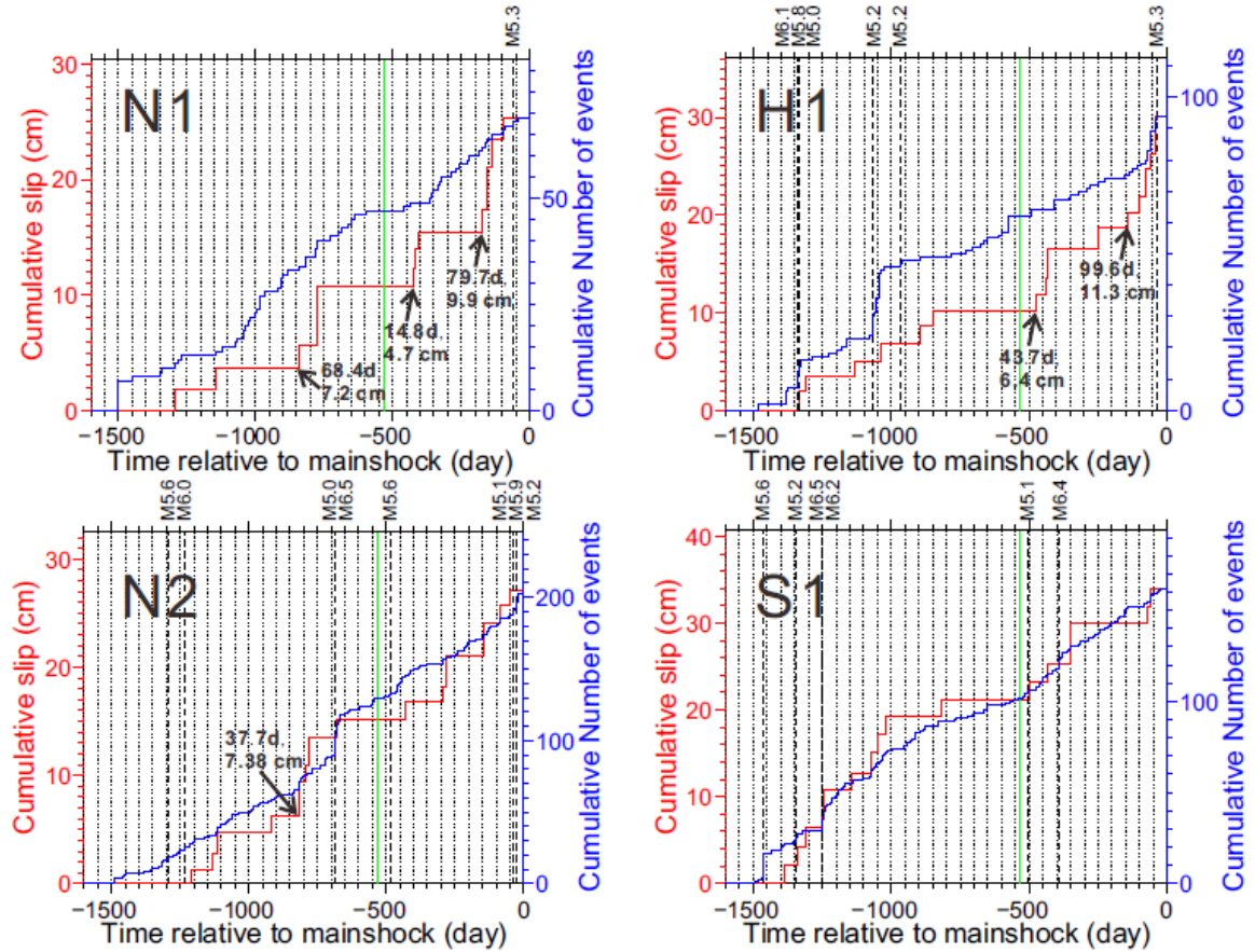
Figure 2. The cumulative number of seismicity (blue curves, M \geq 3.5 ) and average cumulative aseismic slip (red curves) inferred from M \geq 3.0 repeaters within the different regions shown in Figure 1b. Black vertical dashed lines denote M \geq 5.0 events. The green line indicates the timing of the 1 April 2014 M 8.2 Iquique earthquake. The arrows mark the several short-duration aseismic-slip transients with durations and accumulated slip labeled aside.
